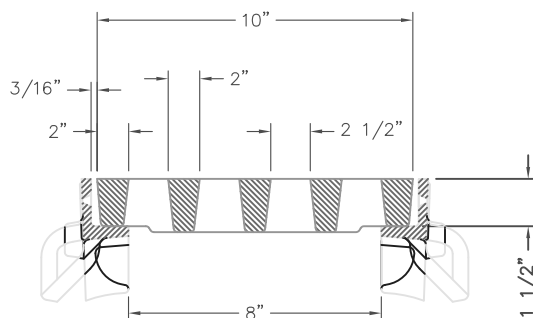
R-4999-BX TYPICAL SECTION TYPE "C" GRATE w/ TYPE "B" FRAME (SCALE: 1/4"=1")
